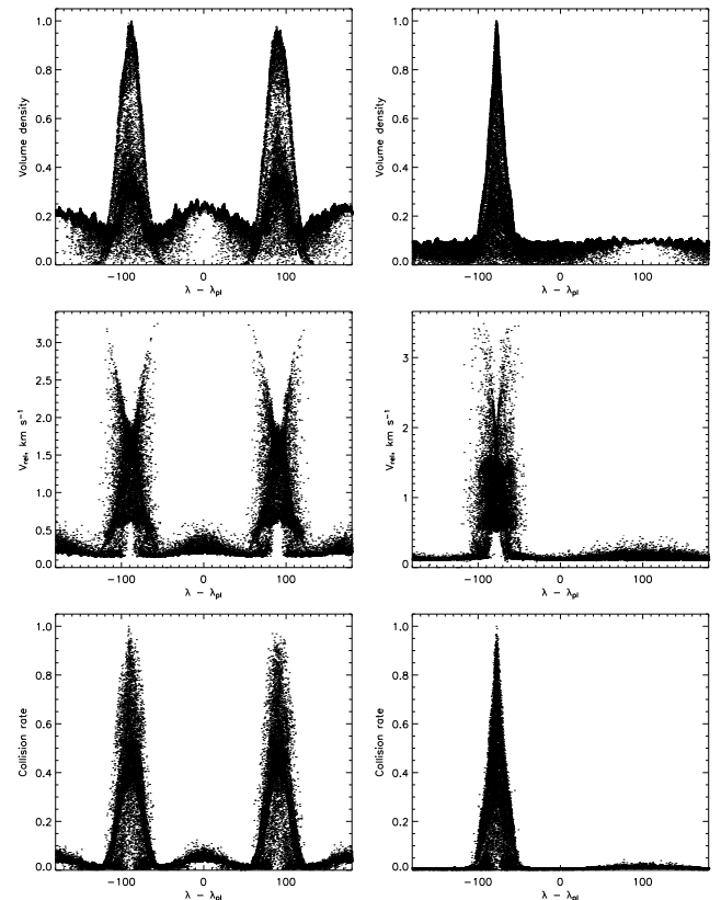
FIG. 4.— Collision rates amongst populations of planetesimals trapped into resonance with a 30M_\oplus planet that migrated 45-60 AU from a 2.5M_* : (left) 3:2 resonance; (right) 2:1(u) resonance. The collision rate (bottom) is the product of the volume density of cross-sectional area of planetesimals (top) and the relative velocity of collisions (middle). Volume densities and collision rates have been normalised to the maximum for all planetesimals. Each point represents the result for one of 40,000 planetesimals in the disks, and is plotted against with the longitude of the planetesimal relative to the longitude of the planet.
