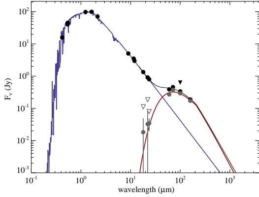
Figure 4. SED for \kappa CrB (Bonsor et al. 2013). Photometry is shown as black dots or black triangles for upper limits. Disc (i.e. photosphere- subtracted) fluxes and upper limits are shown as grey dots and open triangles. The stellar spectrum is shown as a blue line and the red line shows a black-body fit to the disc emission, modified at long wavelengths to illustrate the decrease in emission of more realistic grains. The disc has a black-body temperature of 72 \pm 3 K, which corresponds to a black-body radius of 53 \pm 5 AU. This is subtly different from Bonsor et al. (2013), where \lambda_0 and \beta were free parameters.
