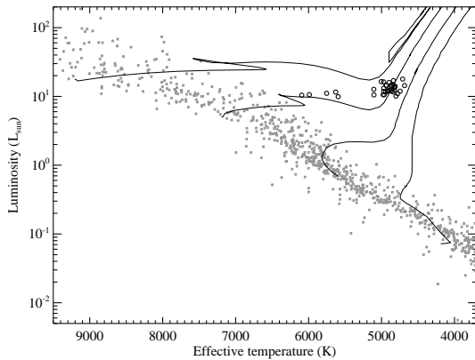
Figure 1. Our sample plotted on a HR diagram (large black circles), alongside stars from the UNS sample (small grey dots), an unbiased sample of nearby main-sequence stars (Phillips et al. 2010) and stellar evolution tracks taken from Girardi et al. (2002) for 0.6, 1, 1.5, and 2.0 M_{\odot} . Tracks start at the zero-age main-sequence and move to the upper right over time. Our sample of subgiants have similar luminosities to main-sequence A stars, but are cooler.
