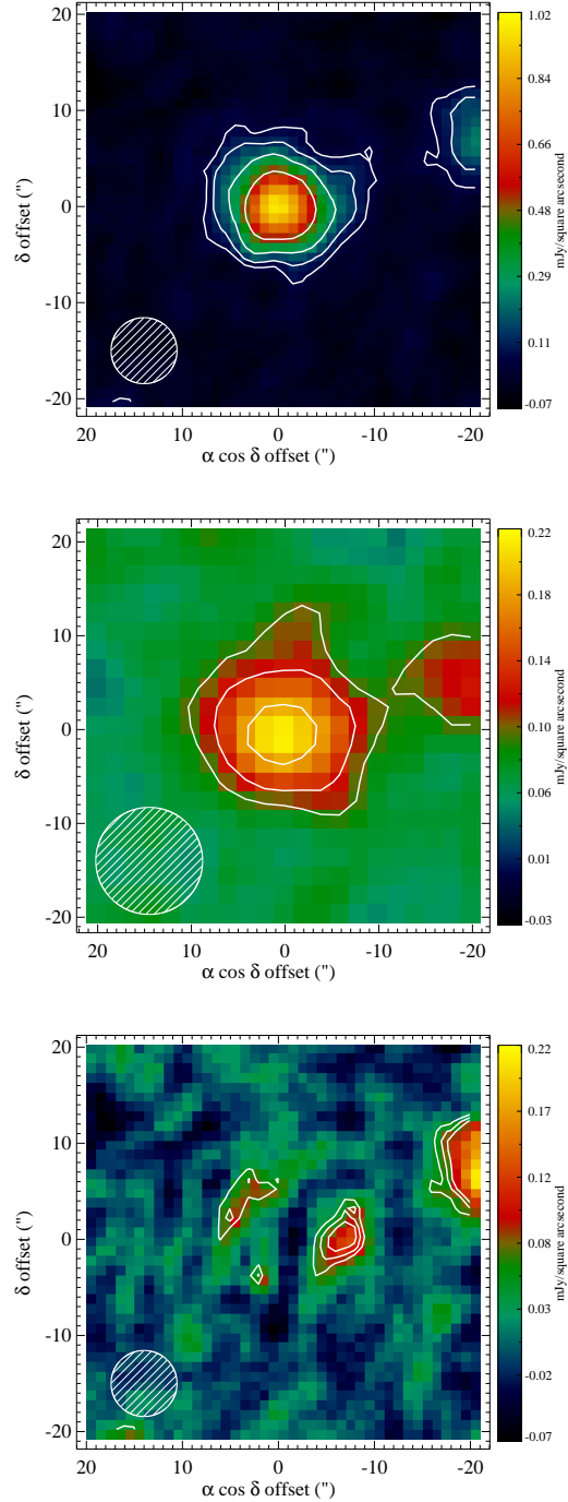
Figure 6. The Herschel images of HR 8461 at 100\mu\text{m} (top) and 160\mu\text{m} (middle), with contours showing detection levels of 3, 6, 12\sigma , where \sigma = 2.09 \times 10^{-5} at 100\mu\text{m} and \sigma = 5.7 \times 10^{-5} at 160\mu\text{m} . The bottom panel plots the residuals after subtracting a stellar PSF scaled to the peak, with contours at 3, 4, 5\sigma . This shows that the disc is marginally resolved at 100\mu\text{m} . A similar plot shows that it is not resolved at 160\mu\text{m} .
