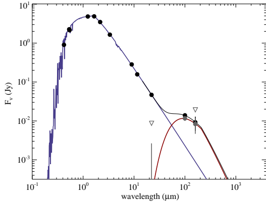
Figure 7. SED of HD 208585, plotted in the same manner as Fig. 4. The disc emission is not well constrained, but we fit a black-body temperature of 56^{+65}_{-30} K, which corresponds to a black-body radius of 94^{+440}_{-20} AU.
