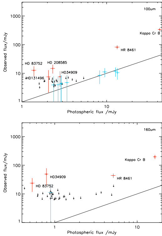
Figure 2. The photospheric flux, predicted using stellar models (as discussed in §3.1) compared to the observed flux at 100\mu\text{m} (top) and 160\mu\text{m} (bottom). The red points show 3\sigma detections of an excess, the blue points, 3\sigma detections of the system, both with 3\sigma error bars, and the black arrows the 3\sigma upper limits on the observed flux, when the detection is below 3\sigma .
