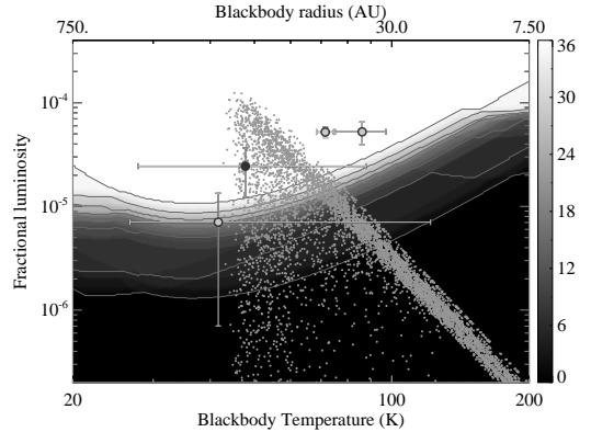
Figure 10. The cumulative detection limits for discs orbiting all of the stars in our sample, as a function of the disc black-body temperature and fractional luminosity (ratio of the total disc luminosity to the total stellar luminosity), with 1\sigma error bars. The equivalent black-body radius for a disc orbiting a 15L_{\odot} star is plotted on the top axis for reference. The discs that were detected in our sample are plotted by the large circles, empty circles for the planet-hosts and filled circles for the non-planet hosts, whilst the small circles show the model population, as described in §4. It should be noted that there is an artificial upper (lower) limit in radius (black-body temperature), which is imposed by the model population based on the work of Wyatt et al. (2007c).
