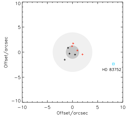
Figure 3. The offset of the centre of the observed emission at 100\mu\text{m} , compared to the nominal location of the star. The grey circles show the weighted average absolute pointing error of our Herschel observations, 1.3'' at 1\sigma and 3.9'' at 3\sigma . The black points show the debris detections ( \kappa CrB, HR 8461, HD 208585 and HD 13496), whilst the red points, show the stars for whom the emission at 100\mu\text{m} was greater than 3\sigma above the error on the observations. The blue square shows HD 83752, whose excess emission is suspected of being contaminated with background emission. The emission surrounding HD 34909 is not point-like and, therefore, omitted from this plot
