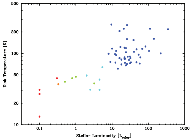
FIG. 3.—Observed temperatures of debris disks vs. stellar luminosities. The A stars (dark blue) are a sample of 46 detected at both 24 and 70 \mu\text{m} (Wyatt et al. 2007). The data for the F (light blue), G (green), K (orange), and M stars (red) are taken from (Lestrade et al. 2006 and references therein), with the addition of TWA 7 from Matthews et al. (2007).
