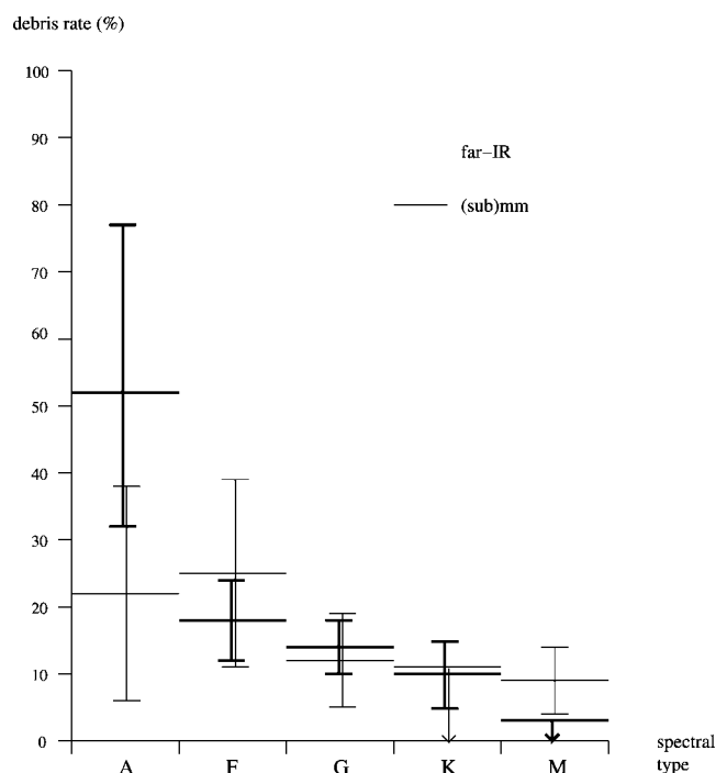
FIG. 1.—Frequency of debris disks as a function of spectral type based on existing data. The error bars are presently large for several spectral types. It is also evident that the submillimeter is the best wavelength range for searching for disks around later type stars. This is consistent with the detection of cold disks. The references for the data are N. Phillips et al. (2007, in preparation), Gautier et al. (2007), Su et al. (2006), Beichman et al. (2005, 2006a), Bryden et al. (2006), Lestrade et al. (2006), Najita & Williams (2005), Liu et al. (2004), Wyatt et al. (2003), and Holmes et al. (2003).
