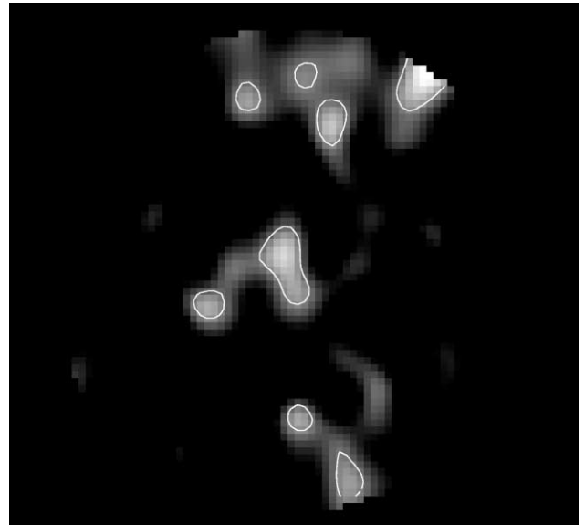
FIG. 4.—Example of disk extraction (Greaves et al. 2004b): disk detection toward \tau Ceti with SCUBA at 850 \mu\text{m} . The rms in this map is 0.7 mJy (per smoothed 20" beam). The faintest detected peaks are 2 mJy beam ^{-1} . The disk is recognized by its elliptical shape centered about the star. This star is nearby, but the disk is in fact one of the smallest yet measured. In addition, this field is unusually rich in background sources.
