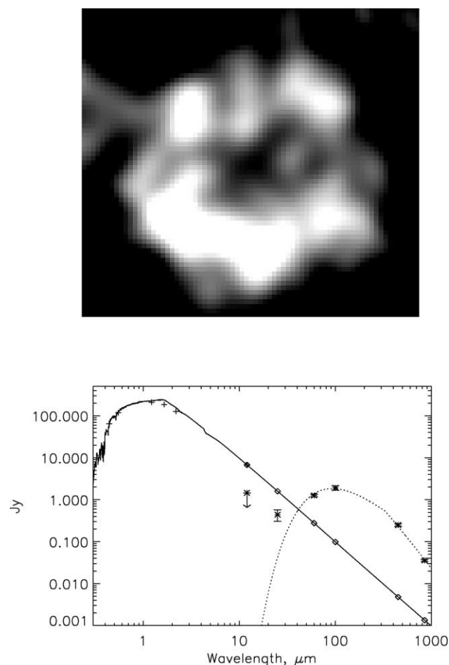
FIG. 2.—An 850 \mu\text{m} image of \epsilon Eridani (Greaves et al. 2005) and the SEDs of the star (solid line) and gray-body fit to the dust (dotted line). Note the much greater disk-to-star contrast in the submillimeter compared to 60 \mu\text{m} , even for this midrange temperature of 55 K.
