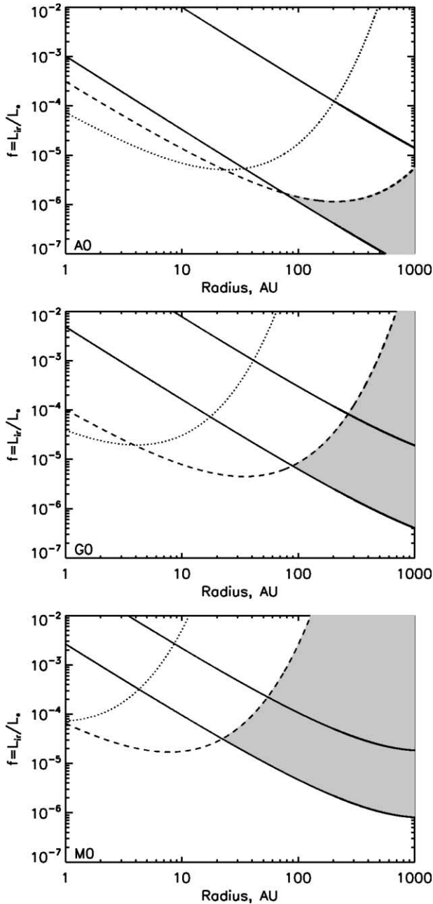
FIG. 6.—Parameter space in which the SCUBA-2 survey is uniquely sensitive ( shaded area ). In each case, this is the location of cold dust. The different lines show the limits of Spitzer 24 \mu\text{m} sensitivity ( dotted line ) assuming a limit of F_{\text{disk}}/F_* = 0.1 , and Spitzer 70 \mu\text{m} sensitivity ( dashed line ) assuming a limit of F_{\text{disk}}/F_* = 0.55 , based on Su et al. (2007). The solid lines are the SCUBA-2 3 \sigma limits for the closest and farthest stars in the samples, assumed to be 2.6–45.2 pc for A0, 3.6–24.8 pc for G0, and 1.8–8.6 pc for M0. For A0 stars, this space is relatively narrow (as shown by the shaded region). However, for M stars, the region is much more extensive and includes significantly smaller disks below the detection limits of Spitzer at 70 \mu\text{m} . This figure does not account for the fact that at these distances, the largest disks are going to be significantly resolved, and therefore we will not reach the 2 mJy limit (i.e., the SCUBA-2 limits are optimistic for disks larger than the beam size).
