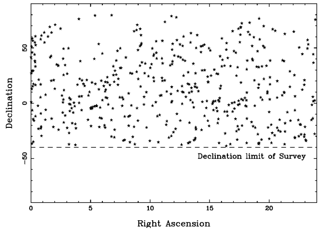
FIG. 7.—Distribution of target sources in the debris disk survey. The targets are all-sky. The declination limits are -40 < \delta < +80 .
