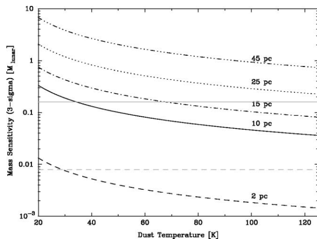
FIG. 5.—Disk mass sensitivity ( 3 \sigma ) as a function of dust temperature for various limiting distances. The outer bound of the A stars sample is roughly 40 pc. The limits for F and G stars are \approx 25 pc, and all the M stars lie within the 10 pc boundary. The horizontal lines show the mass of the \epsilon Eridani disk (solid line) and 10 times the mass of the Kuiper Belt (dashed line). An opacity of 1.7 \text{ cm}^2 \text{ g}^{-1} is adopted.
