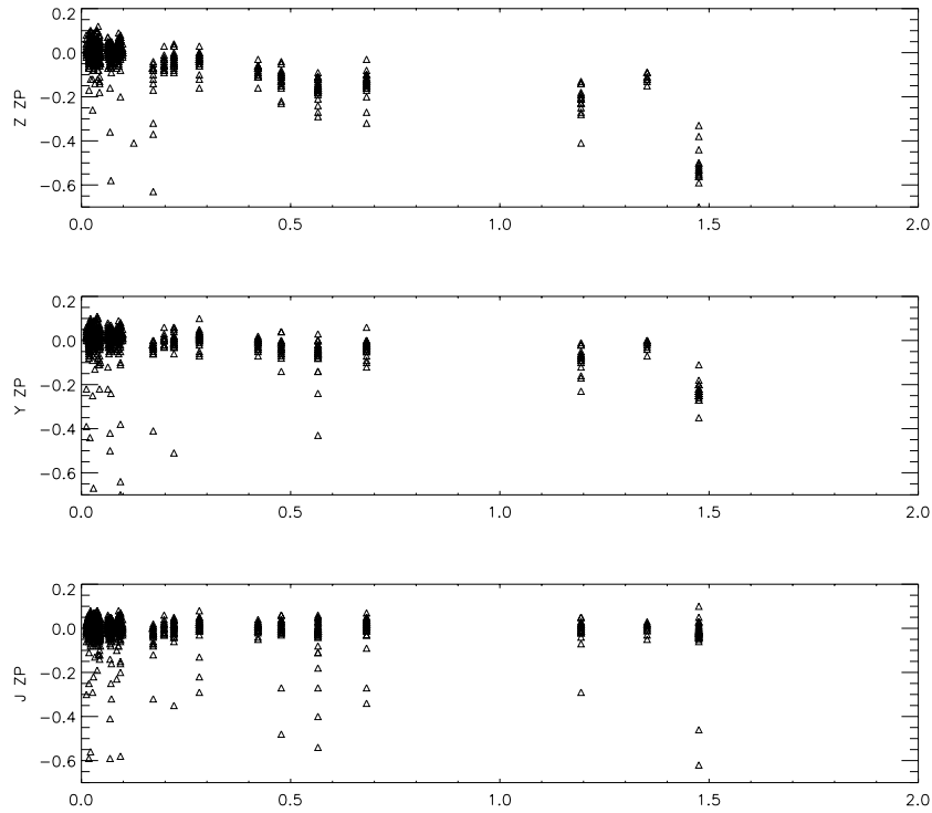
Figure 10: \Delta zerpoint versus corrected E(B-V) for the ZYJ filters for all photometric nights in 05A and 05B.
