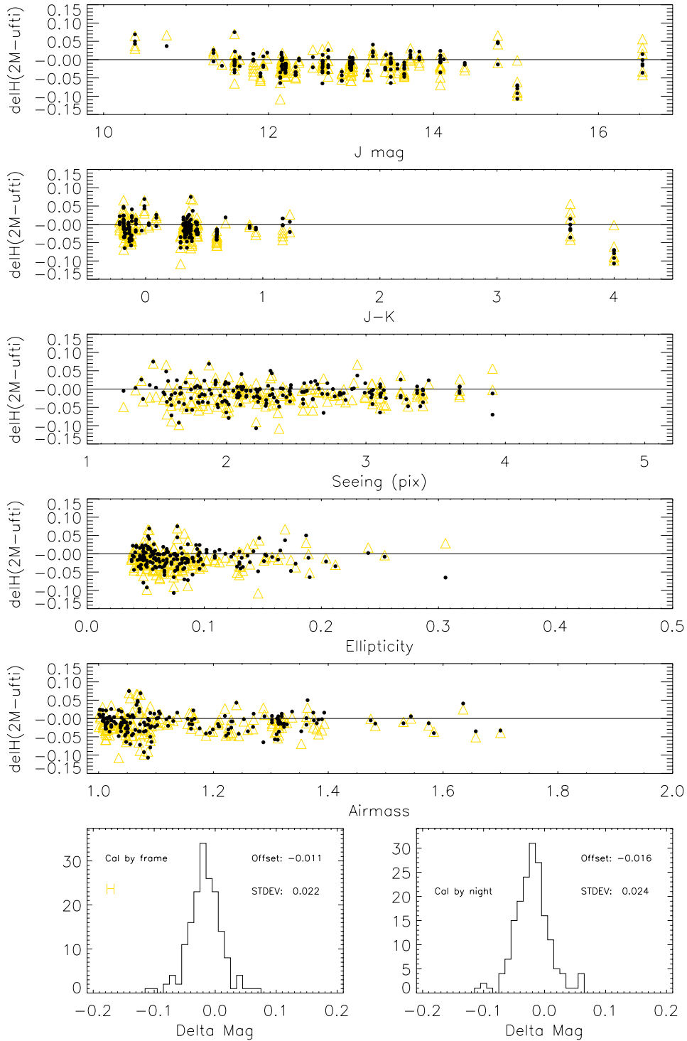
Figure 3: H-band \Delta\text{mag} (2MASS calibration-UFTI) for UKIRT faint standard stars observed with WFCAM. Measurements calibrated with a per-frame zeropoint, MAGZPT, are black dots, while measurements calibrated with a by-night zeropoint are yellow triangles. The histograms at the bottom collapse the data along the Y-axis for the by-frame (LHS) and by-night (RHS) calibrations.
