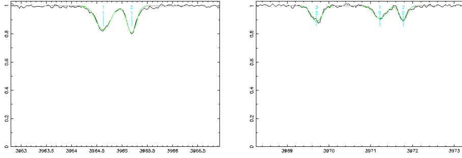
Figure 3: A three component Ly \alpha fit to a region of the sample spectrum, obtained using the methods described in the text. Fits at redshift z = 1.561 to CIV 1548 (left) and CIV 1550, with low redshift to Galactic CaII 3970 (right).
